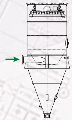
T - TANGENTIAL INLET
